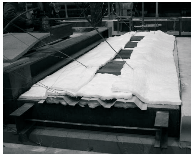
Fig. 4: The tested specimen before the fire experiment
