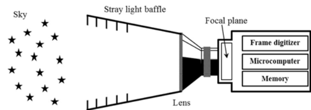
Fig. 1: Principle sketch of a second generation star tracker
