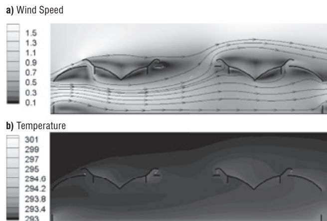
FIGURE 4. Simulated contours for (a) wind speed ( \text{m s}^{-1} ) and (b) temperature distribution ( ^{\circ}\text{K} ) for the M3S2 simulation.
