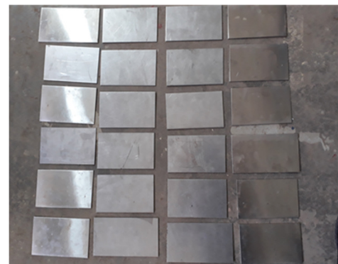
Fig 1. Weld specimen's preparation.
