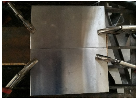
Fig. 2. Workpiece sheets before and after welding process.
