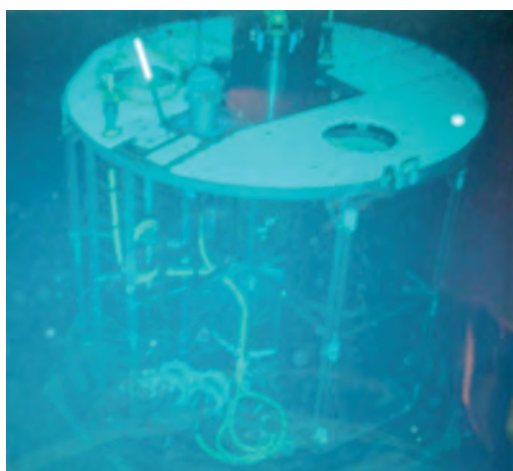
Fig. 8. Borehole observatory.
