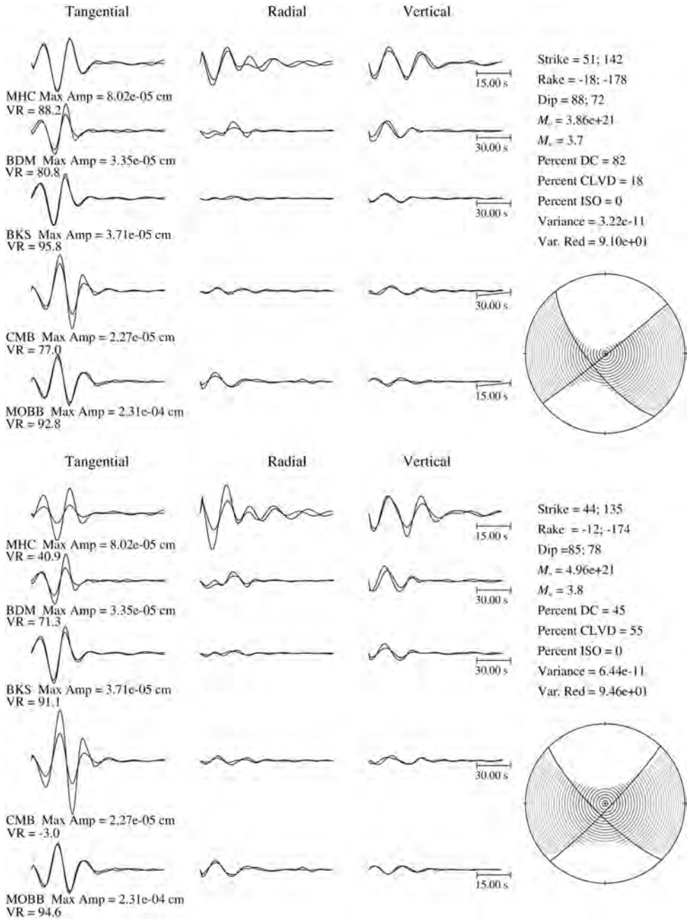
Fig. 15. Results of moment tensor inversions for the M 3.63 regional event shown in fig. 14. Top : inversion using 4 stations of the BDSN and MOBB (BDM, BKS, CMB are bandpass filtered between 0.02 and 0.05 Hz; MHC and MOBB, between 0.05 and 0.10 Hz). Bottom : results of inversion using only MOBB, showing the good fits of the single station solution to the other BDSN waveform data.
