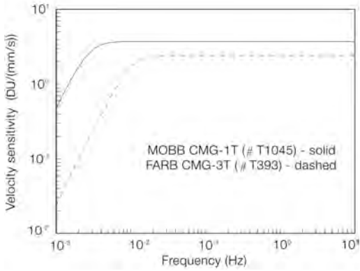
Fig. 8. Comparison of instrument responses of the CMG-1T at MOBB and the CMG-3T at FARB.
