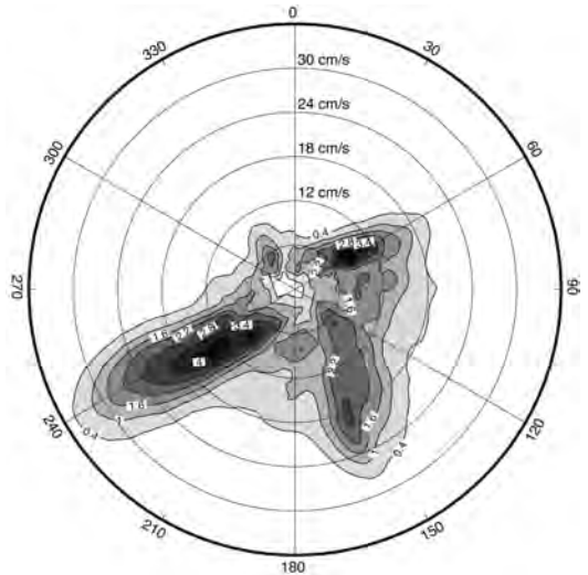
Fig. 10. Distribution of current velocity data as a function of azimuth for the 78-day period shown in fig. 9. The contour label units are fractions of the average density distribution of the current velocity. The two dominant maxima (centered at 60° and 240°, i.e. orthogonal to the continental shelf) are associated with the semi-diurnal tidal currents. The third directional peak is roughly parallel to the coastline and appears to be related to the dominant ocean circulation.
