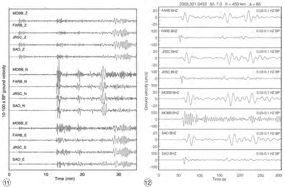
Fig. 11. Comparison of vertical, N and E component records of the 26/04/2002 M_w 7.1 Mariana earthquake (depth = 85.7 km, distance = 85.2°, azimuth = 283° from MOBB), at MOBB and 3 stations of the BDSN. The records have been band-pass filtered between 10-100 s.
