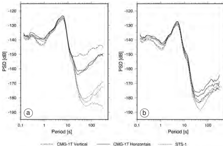
Fig. 3a,b. Comparison of typical background noise PSD levels observed by the CMG-1TD and the co-sited STS-1's in the BKS vault, a) before and b) after it had been installed in the titanium pressure vessel, appropriately insulated and purged with argon gas. The large dashed line and the solid lines are the Z component and horizontal component PSD's, respectively, and the small dashed lines are the STS-1 PSD's. Note that the CMG-1TD PSD levels are within \sim 5 dB of the STS-1 PSD levels at long periods after insulation (Uhrhammer et al. , in prep.).
