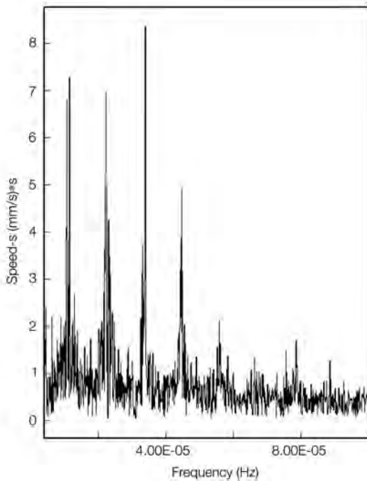
Fig. 9. Spectrum of current speed [units are (mm/s)/ Hz] based on a 78-day period of current meter data. The four dominant group of peaks coincide precisely with the frequencies of the diurnal, semi-diurnal, 8 h and 6 h components of the gravitational tides.
