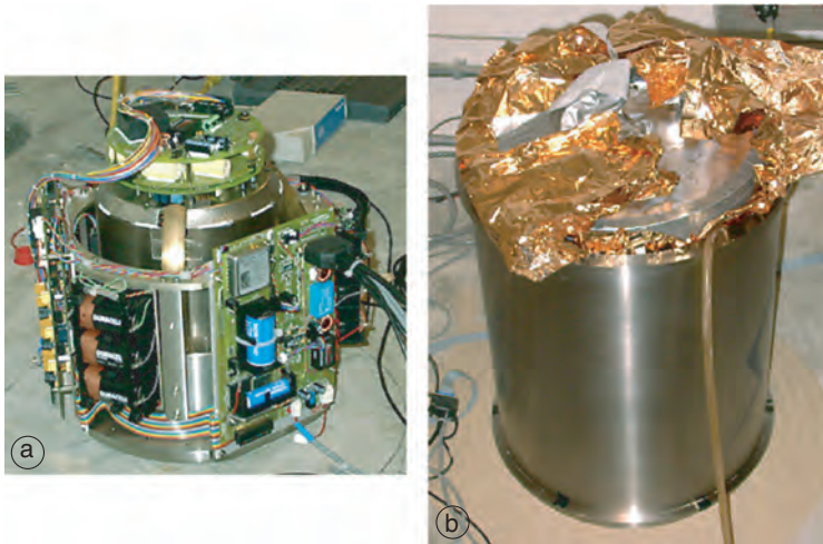
Fig. 2a,b. a) Photo of a Guralp CMG-1TD seismometer in the Byerly Vault (BKS). Shown are the various circuit boards on the sides and the top of the sensor package. Three of the nine batteries used by the leveling system are on the left front and the system clock is on the circuit board on the right. The seismometers are in the \mu metal shielded container mounted on leveling gimbals in the center. b) Photo of the titanium pressure vessel containing the CMG-1TD and resting on a \sim 1 cm thick bed of kiln dried fine sand on the concrete pier at BKS, for the purpose of noise comparisons (Uhrhammer et al. , in prep.).
