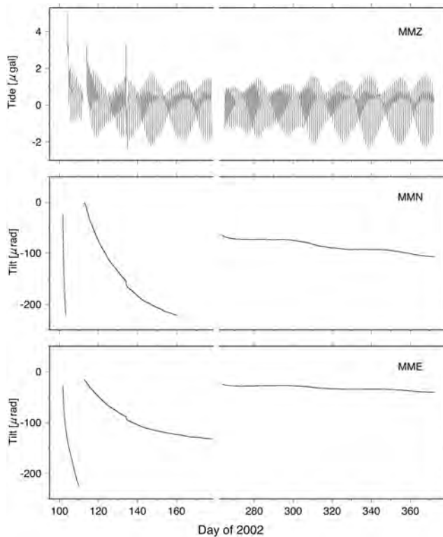
Fig. 5. Mass position data, for portions of the time period 11/04/2002–07/01/2003, showing the progressive settling of the seismometers. At periods longer than the free period of the seismic sensor, the mass position is proportional to tilt on the horizontal components, and to perturbations in gravity on the vertical component. The mass position has therefore been converted to acceleration (vertical component, MMZ) and tilt (horizontal components (MMN, MME)). The large steps on the horizontal components are associated with: 1) installation (day 100); 2) re-centering (day 112, day 263). There is a smaller step on day 134, associated with a local M_w 4.95 earthquake. The vertical component data have been detrended by subtracting a running 36 h average ( \pm 18 h) from each 1/2 h duration smoothed data sample, to bring out the clearly visible tide signal.
