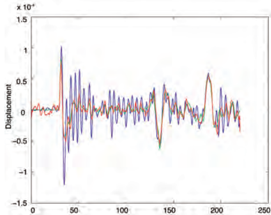
Fig. 13. Raw vertical component data ( P -wave and depth phases) observed on the vertical component at stations MOBB (blue) and JRSC (green) for the 17/11/2002 deep Kurile Island earthquake. Clearly seen is the ringing due to the soft sediment layer in Monterey Bay. The red trace shows the MOBB data after removal of the transfer function constructed using JRSC data.
