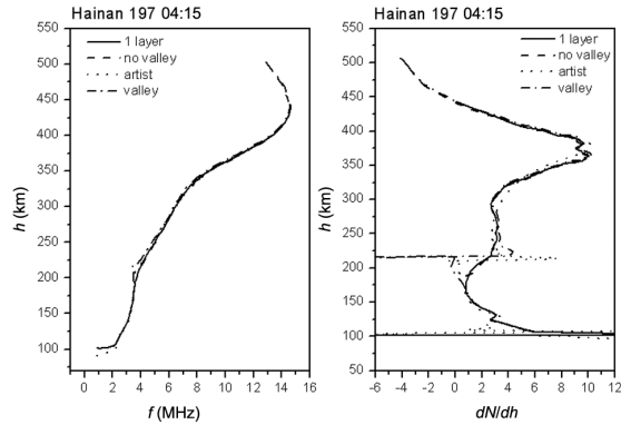
Fig. 1. Electron density profiles and first derivatives dN/dh with different inversion techniques for day 197 and hour 04:15 UT corresponding to Hainan link.
