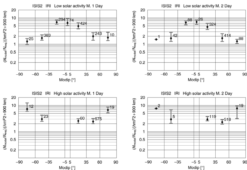
Fig. 6. Comparison of electron density, IRI model, 900 km above hmF2 for months groups 1 and 2. Numbers indicate the amount of data.
