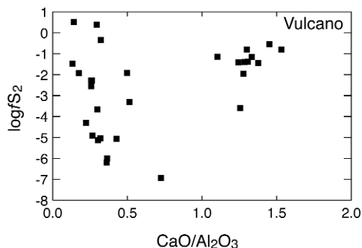
Fig. 6. Evolution of fS_2 with CaO/Al_2O_3 ratio of Vulcano magmas. The fS_2 is calculated from melt inclusion data (Clocchiatti et al. , 1994a,b; Giocada et al. , 1998) and eq. (2.1) (see text). Note that the most primitive melts (high CaO/Al_2O_3 ratio) cluster at around fS_2 of 0.1 bar, whereas the rest of melts defines a negative trend of increasing fS_2 with differentiation.
