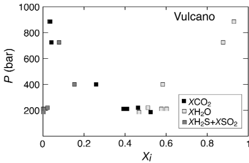
Fig. 12. Composition of fluids in equilibrium with melt inclusions of Vulcano magmas (Clocchiatti et al. , 1994a,b; Gioncada et al. , 1998). X_i is the mole fraction of species i . Fluid compositions have been calculated assuming that the melt inclusions contain 50 ppm dissolved \text{CO}_2 . This gives maximum \text{CO}_2 contents of the fluid. Note the continuous evolution of the fluid composition with pressure.
