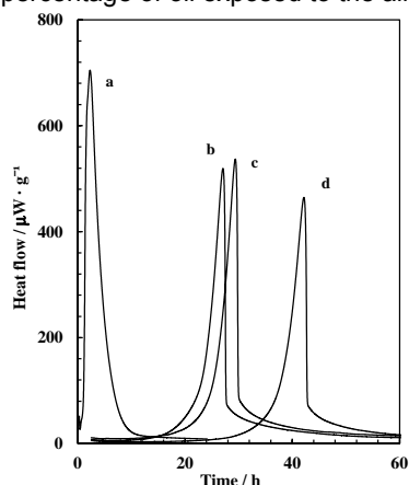
Figure 1: Effect of PGSS encapsulation on the oxidative stability of linseed oil as a function of the processing pressures: a, linseed oil; b, linseed oil encapsulated at 30 MPa; c, linseed oil encapsulated at 20 MPa; d, linseed oil encapsulated at 10 MPa
