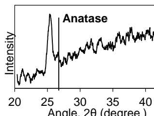
Figure 2: X-Ray diffraction pattern of N-doped \text{TiO}_2 coating film deposited on stainless steel with 6 coating cycles
