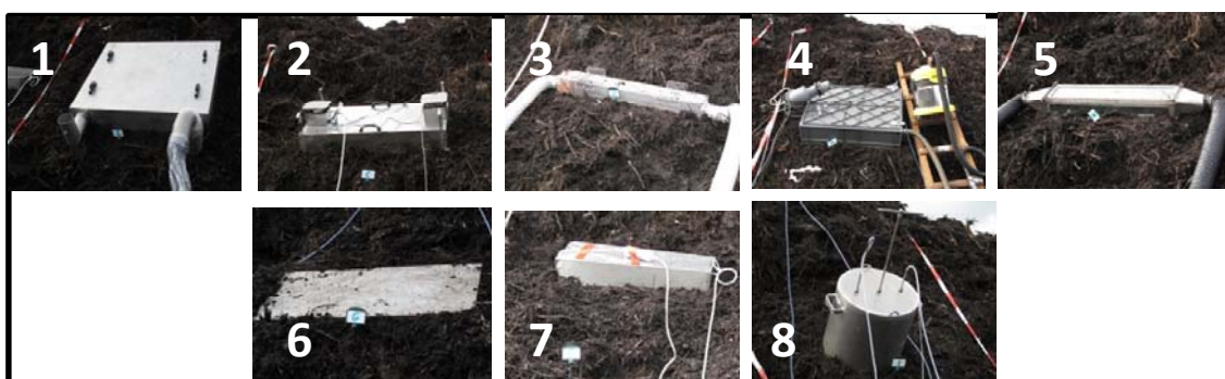
Figure 1: Pictures of the eight sampling devices used on solid source (composting pile). High flow tunnels are numbered from 1 to 5 and low flow chambers from 6 to 8.
