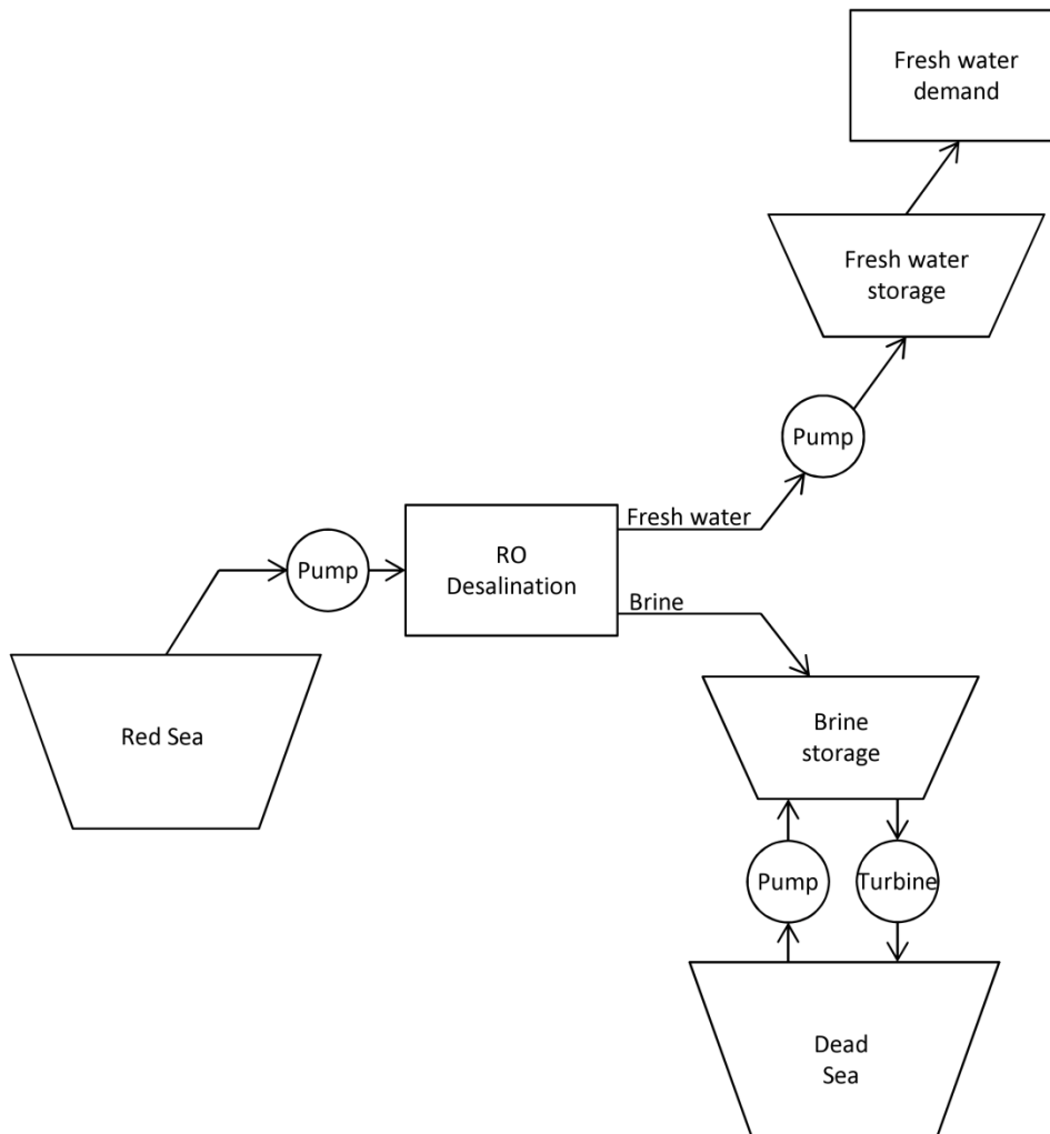
Figure 3: Desalination system
