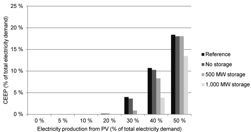
Figure 5 CEEP in relation to electricity production from PV
