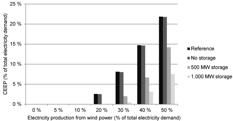
Figure 4 CEEP in relation to electricity production from wind power
