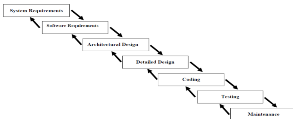
Gambar 1. Waterfall model.
