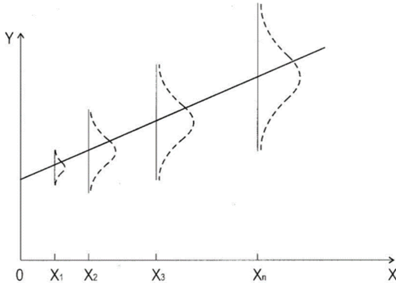
Figure 1. Heteroskedastic errors
