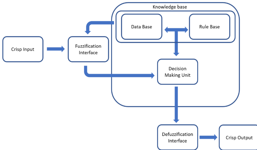
Figure 1. Fuzzy inference system
