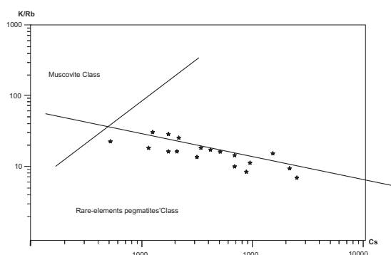
Figure 4: Plots of K/Rb Versus Cs for The Pegmatites' Muscovites.
