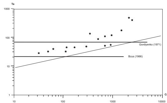
Figure 5. Plot of Ta Versus Cs For The Muscovites of Nasarawa Pegmatites.
