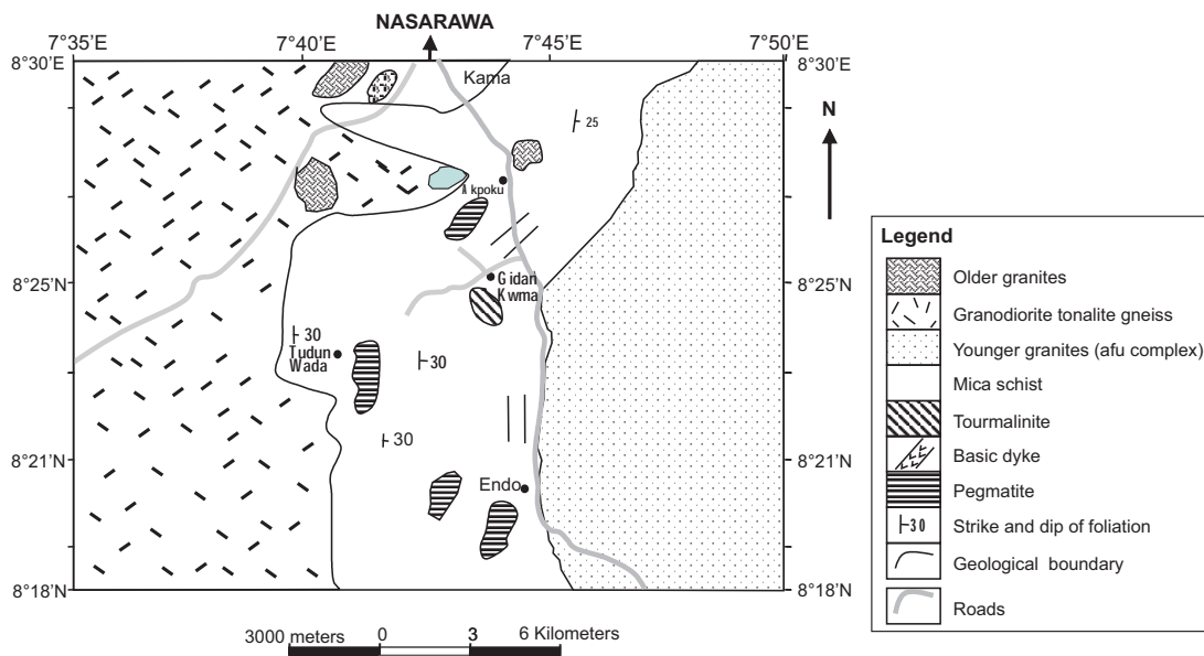
Figure 2: Geological Map of Nasarawa Area.
