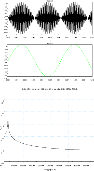
Fig. 8. Time-domain and Frequency-domain responses for DSB signal
