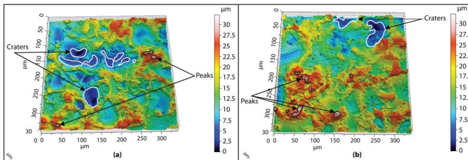
Fig. 7 3D surface stereogram of Ti-6Al-4V alloy after machining at (a) I_p=7 A, T_{on} = 10 \mu s, T_{off} = 30 \mu s and C_p=4 g/l and (b) I_p=7 A, T_{on} = 10 \mu s, T_{off} = 50 \mu s and C_p=20 g/l
