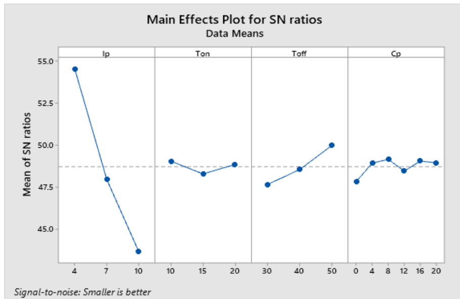
Fig. 4 Effect of process parameters on TWR
