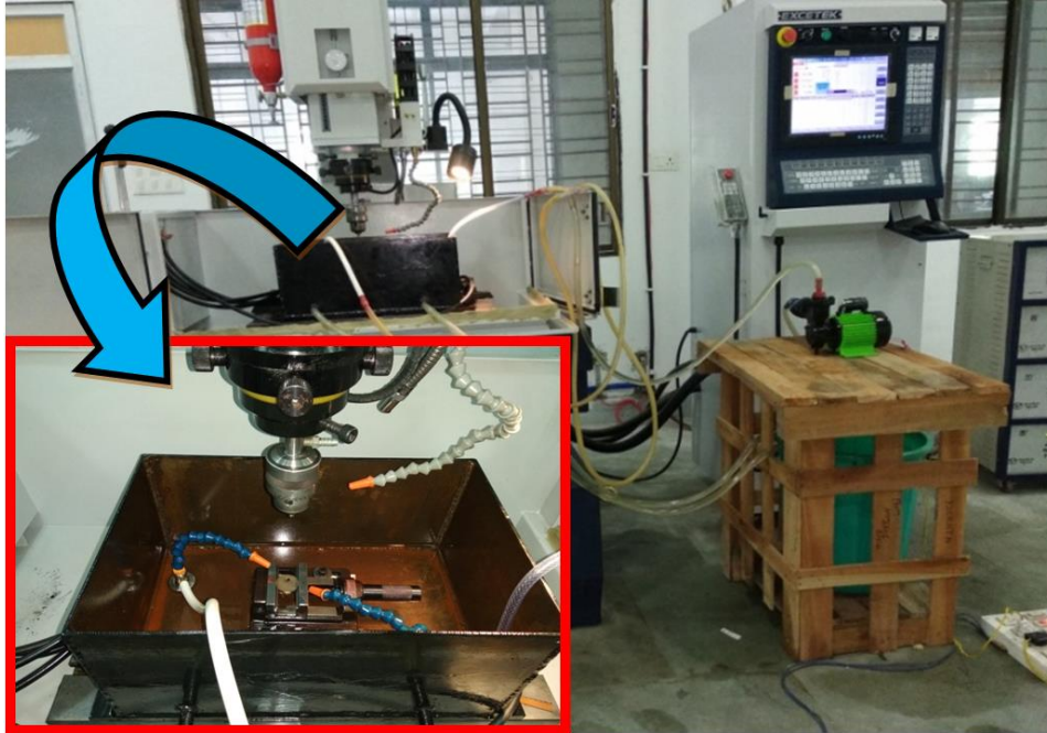
Fig. 2 Newly developed PMEDM experimental set-up
