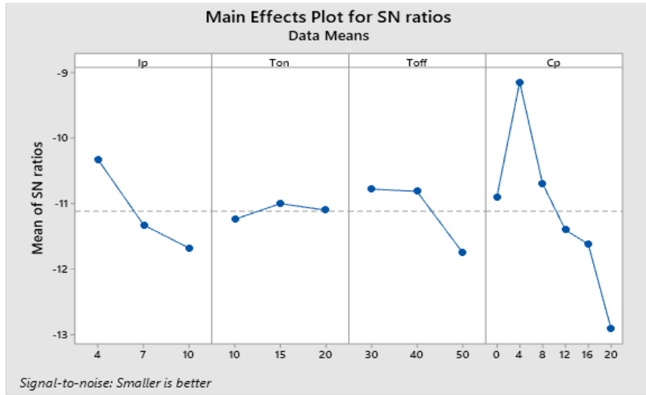
Fig. 5 Effect of process parameters on SR
