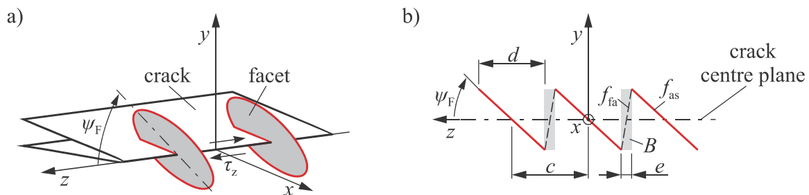
Figure 5: Definition of characteristic dimensions for facet quantification: a) Schematic facet formation at the crack front due to \tau_z , b) Facet's geometry and characteristic dimensions in the y-z-plane
