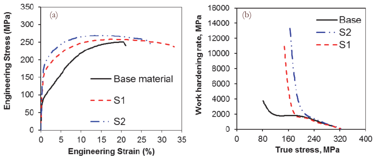
Figure 4: A comparison between base and forged conditions, (a) stress strain curves (b) and K-M plot of the base (as-extruded) and forged AZ31B magnesium alloy during tensile loading.
