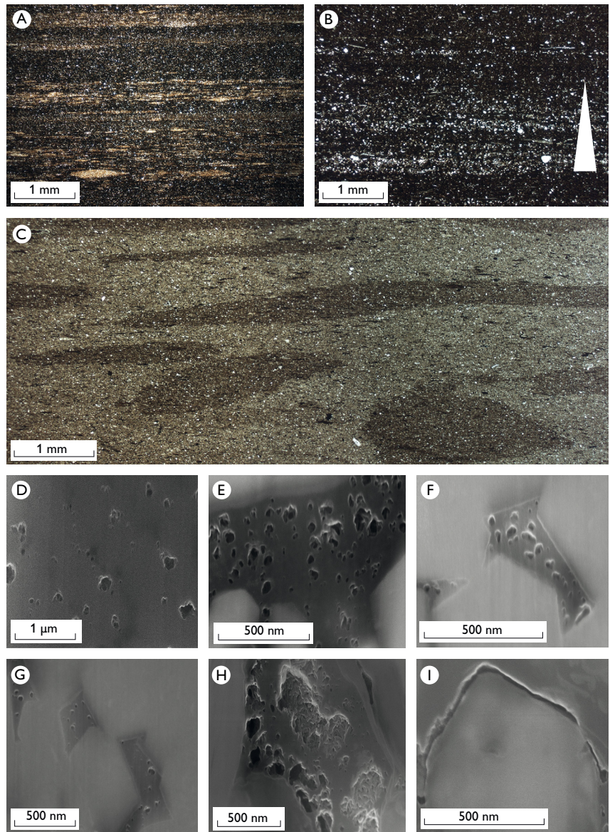
Fig. 4. Micrographs of different mudstone fabrics and pores recognised in the Palaeozoic shales. A: Dark coloured mudstone fabric intercalated with laminae of lenticular clast-rich mudstone fabric, 119.78–119.80 m (Alum Shale Formation). B: Silt-rich mudstone fabric with normal grading, 41.15–41.17 m (Rastrites shale). C: Bio-mottled mudstone fabric, presumably Chondrites , 86.68–86.70 m (Dicellograptus shale). Organic pores: D: Rounded pores, 74.77–75.01 m (Dicellograptus shale). E: Sub-rounded pores, 24.78–24.80 m (Rastrites shale). F: Subrounded to rounded pores in pyrite, 115.63–115.65 m (Alum Shale Formation). G: Subrounded to rounded pores in pyrite, 115.63–115.65 m (Alum Shale Formation). H: Irregularly shaped and complex pores, 24.78–24.80 m (Rastrites shale). Inorganic pores: I: Irregularly shaped pores surrounding silt- to clay-sized grains, 115.63–115.65 m (Alum Shale Formation).
