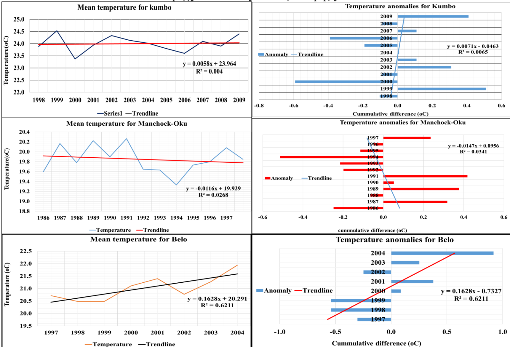
Figur 2: Mean temperature trends and anomalies for the localities of Kumbo, Manchock and Belo Source: Data from the Divisional and Sub delegations of agriculture Bui,Oku and Belo, 2016
