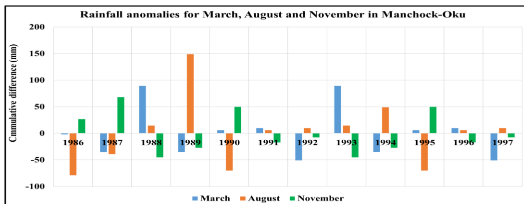
Figure 1: Rainfall anomalies for some key months of bee farming in Manchock-Oku Source: Data from the community forest office Manchock, 2016.
