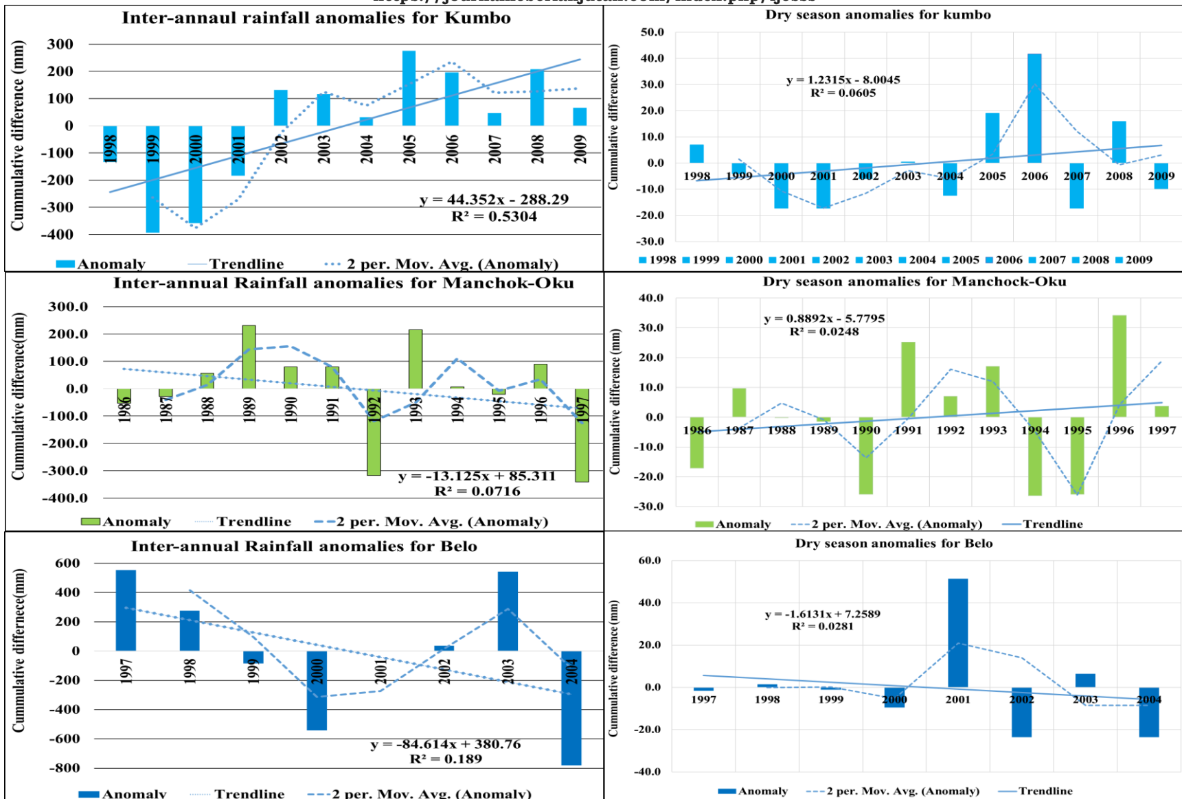
Figure 3: Annual rainfall and dry season rainfall anomalies localities of Mount Oku area Source: Data from the Divisional and Sub delegations of agriculture Bui,Oku and Belo, 2016
