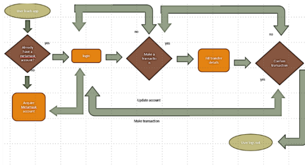
Fig. 3. System Workflow
