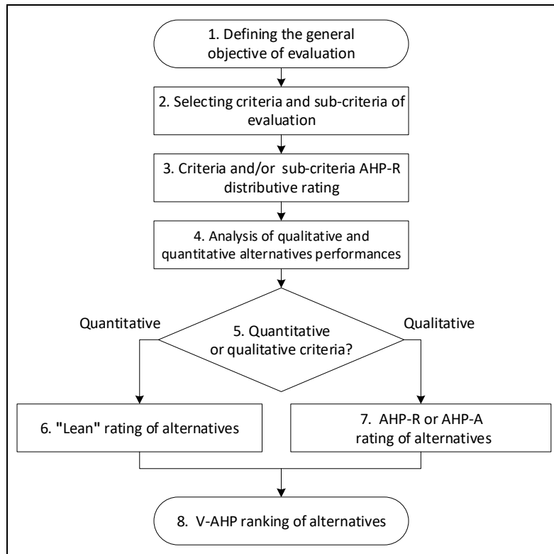
Figure 1 V-AHP procedure
