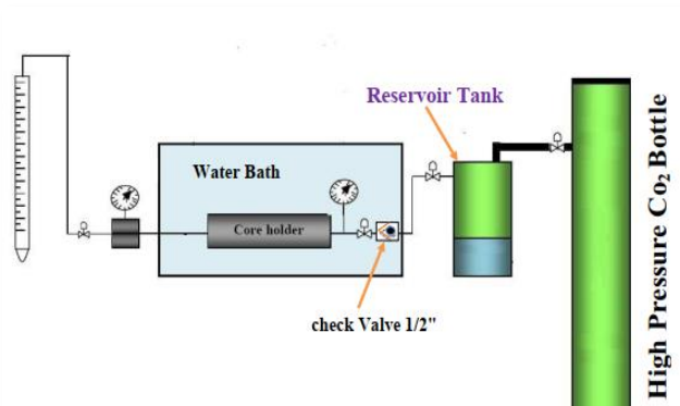
Fig. 1. Fluid injection system design
