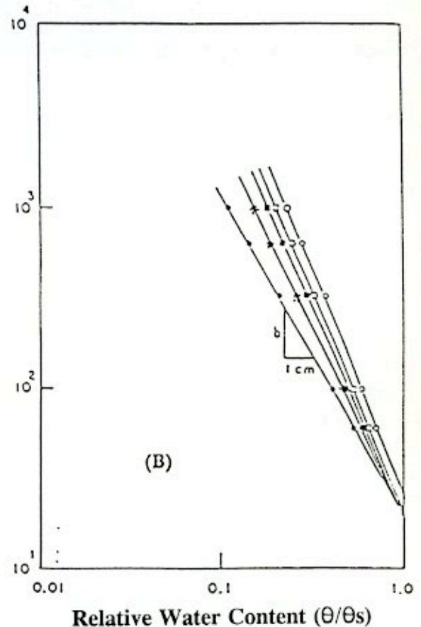
Figure 6. The relationship between the matrix potential and relative water content ( \theta/\theta_s ) as affected by sewage sludge of slightly (A) and moderately (B) calcareous sandy soils
