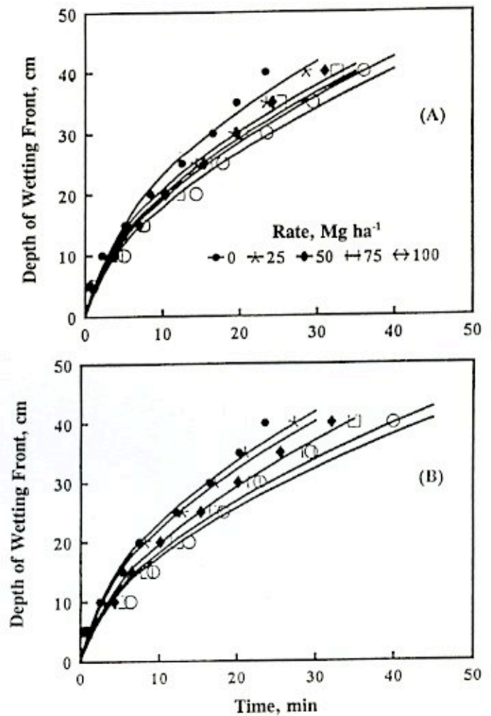
Figure 3. The effect of sewage sludge on advance of the wetting front of slightly (A) and moderately (B) calcareous sandy soils
