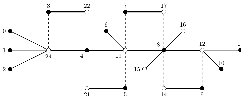
Figure 4. \alpha -labeling of a graph obtained by duplicating some edges of a caterpillar
