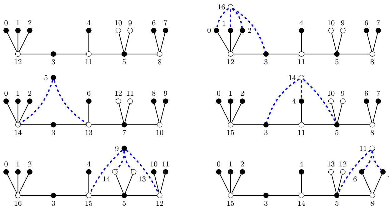
Figure 2. \alpha -labeled graphs obtained by duplicating every internal vertex of a caterpillar
