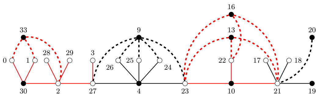
Figure 3. \alpha -labeling of a graph obtained by duplicating multiple vertices of a caterpillar
