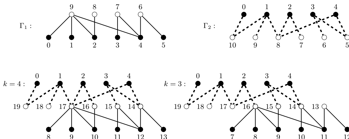
Figure 6. \alpha -labelings of some k -vertex amalgamations of two \alpha -trees
