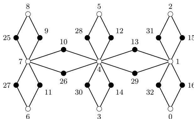
Figure 8. \alpha -labeling of a quadrangular cactus built on an \alpha -tree
