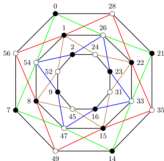
Figure 5. \alpha -labeling of the 3-tie of C_8
