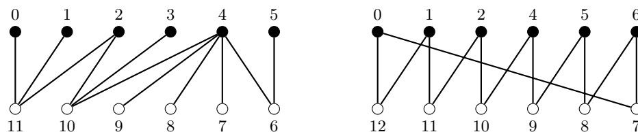
Figure 1. A caterpillar and a cycle with their respective \alpha -labeling
