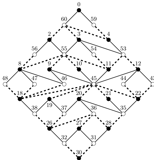
Figure 9. \alpha -labeling of an irregular grid
