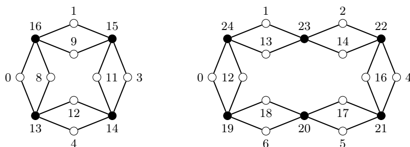
Figure 7. \alpha -labelings of a supersubdivision of C_4 and C_6
