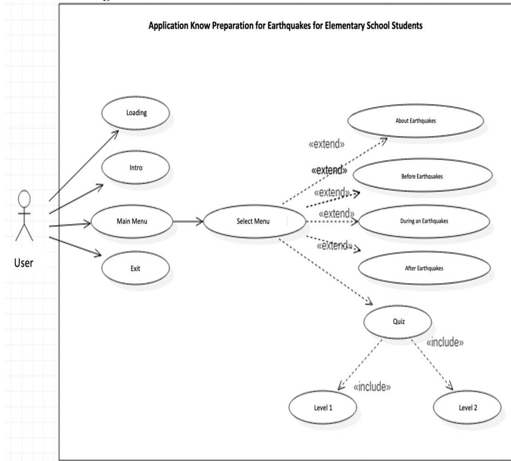
Fig 1. Use Case Diagrams
