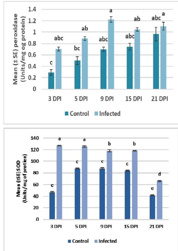
Fig. 3: Response of SOD and POX activity in IIHR-2611 to ToLCBaV infection. Bar charts of different colour and with different letters are significantly different ( P < 0.05 , F = 1.702 , df = 18 , P = 0.021 for POX and F = 3.75 , df = 18 , P = 0.021 ) based on Tukey's HSD test. Data presented as means \pm SE ( n = 3 )
