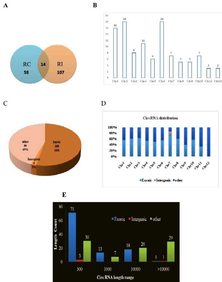
Fig. 1. Identification and characterization of CircRNAs in response to ToLCBaV in a resistant tomato genotype. (A) Number of CircRNAs identified in RC and RI. (B) CircRNAs distribution on each chromosome. (C) The number and percentage of CircRNAs originated from exon, intergenic and other genomic regions. (D). Percent distribution of exonic, intergenic and other CircRNAs across chromosomes. (E) Classification of CircRNAs based on length range.
