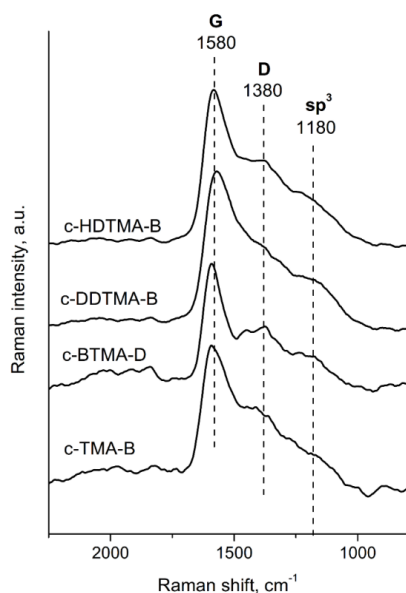
Fig. 3. Raman spectra of c-HDTMA-B, c-DDTMA-B, c-BTMA-B and c-TMA-B in the range between 2200 and 800 \text{cm}^{-1} .
