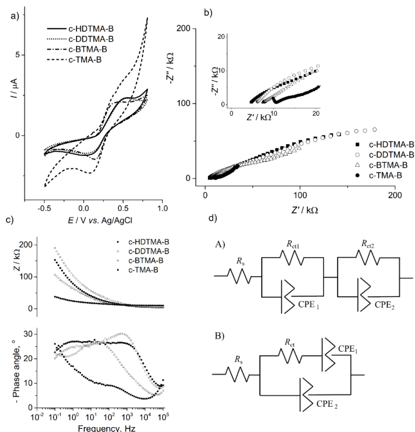
Fig. 4. Carbon paste electrodes modified with different clay samples: a) cyclic voltammograms recorded in 1 mM K_4[Fe(CN)_6] + 0.2 M KCl at a scan rate of 50\text{ mV s}^{-1} ; b) Nyquist plot recorded in the same solution in OCP; c) Bode plot recorded in the same solution in OCP; d) the equivalent electric circuit used to fit EIS data.
