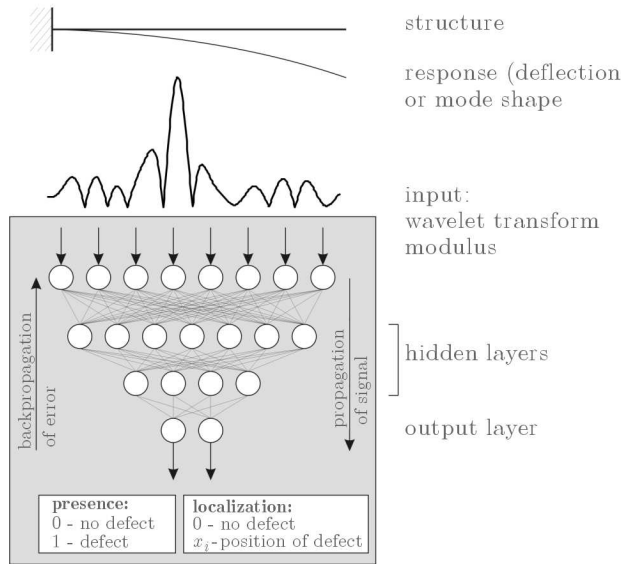
Fig. 2. Outline of the neuro-wavelet damage detection system
