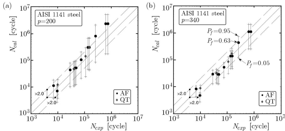
Fig. 6. Comparison of the experimental lives N_{exp} with the calculated lives N_{cal} for (a) p = 200 and (b) p = 340 for the notched round specimens in AISI 1141 steel under fully reversed tension
