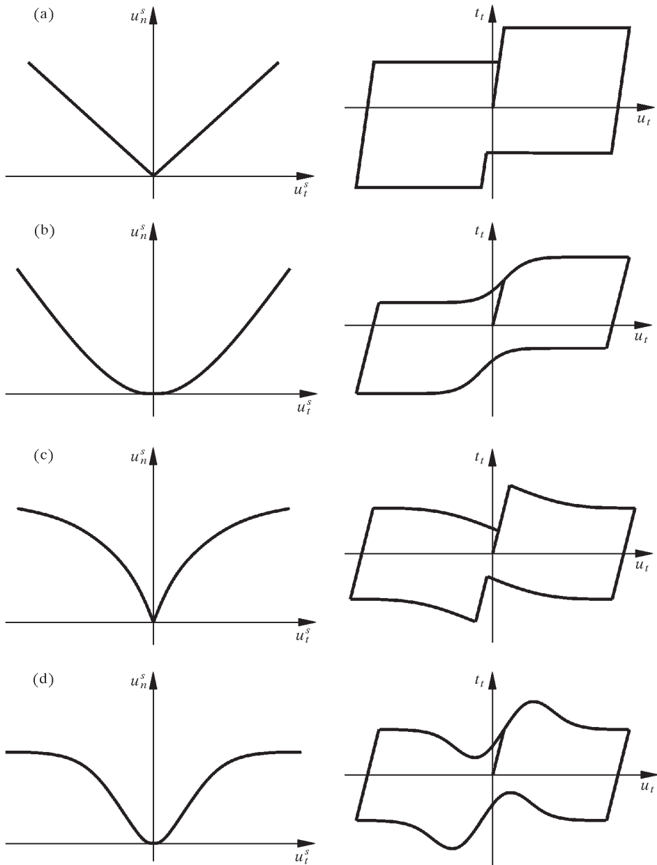
Fig. 17. Configurational dilation: typical dilation curves and resulting cyclic shear response
