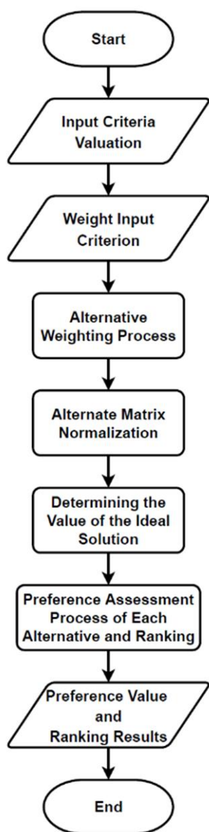
Figure 4. TOPSIS flowchart
