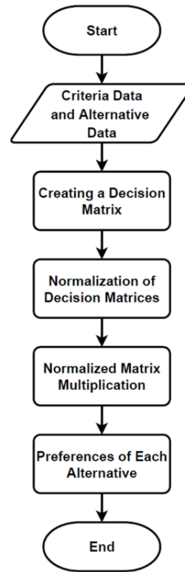
Figure 2. SAW Flowchart
