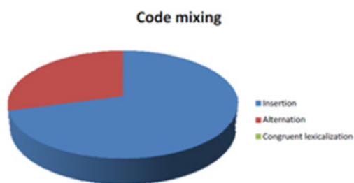
Figure 2 Code-Mixing
