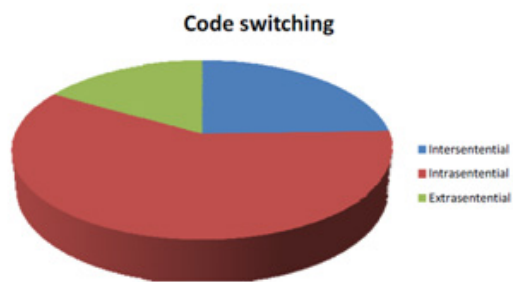
Figure 3 Code-Switching
