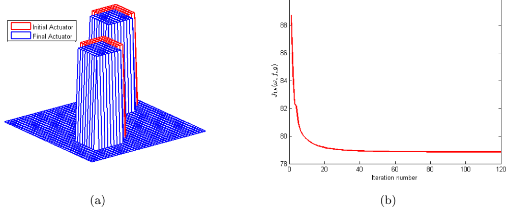
FIGURE 2. (a) The initial actuator center locations: (0.4, 0.4) , (0.825, 0.825) (red) and final actuator center locations: (0.325, 0.325) , (0.75, 0.75) (blue). (b) The history of cost functional J_{1,h} , as the actuators move from the initial to the optimal actuator locations. The speed of the wave is set to c = 1 .
