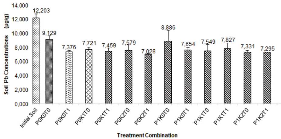
Fig 1 Histogram of soil Pb concentrations.
