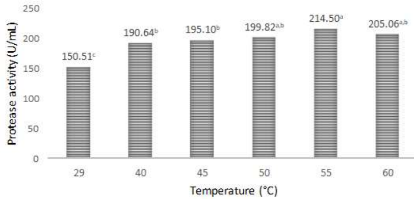
Fig 1 The effect of temperature on the alkaline protease activity of A. flavus DUCC-K225. Remarks: the same superscripts show no significantly difference ( p < 0.05 ).
