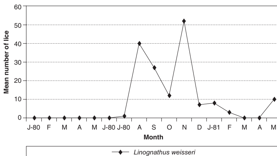
FIG. 4 Seasonal pattern of intensity of infestation of Linognathus weisseri on impalas at Skukuza and in the Mbiyamiti regions, Kruger National Park, South Africa during 1980/81. The monthly sample ranged from 4–13 impalas
