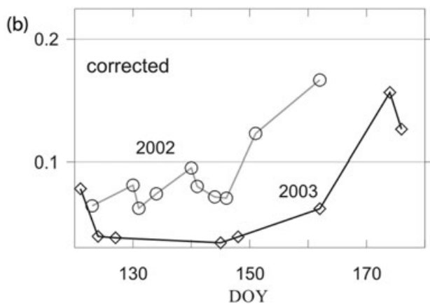
Fig. 4 Time series of the Normalized Difference Snow and Ice Index (NDSII) for 2002 and 2003, between day of year (DOY) 120 (30 April) and 180 (29 June), on fast ice in Kongsfjorden. (a) Top of the atmosphere (TOA) values of NDSII. (b) TOA values corrected for atmospheric water vapour (AWV). Coincident ground measurements were performed in these years.
