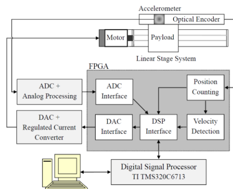
Fig. 2 Schematic of the experimental system
