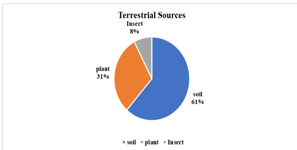
Figure 5. Percentage of terrestrial sources of different Streptomyces species, including soil, plant, and insect.
