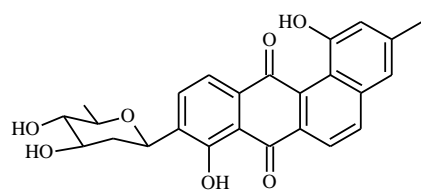
49. Dehydroxaquayamycin
