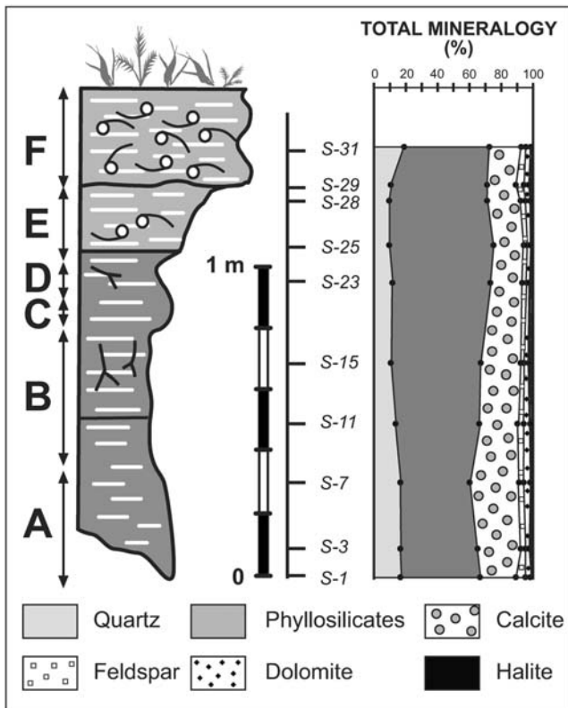
Fig. 2 - Results of the mineralogical (XRD) analysis (%).
